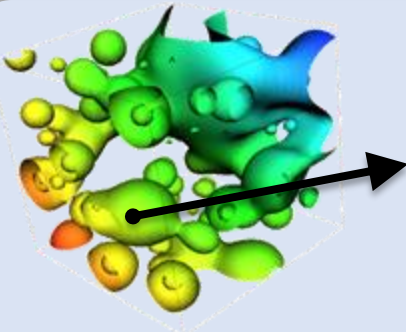
Visual Debugging
