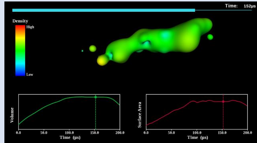
Presentation Graphics
